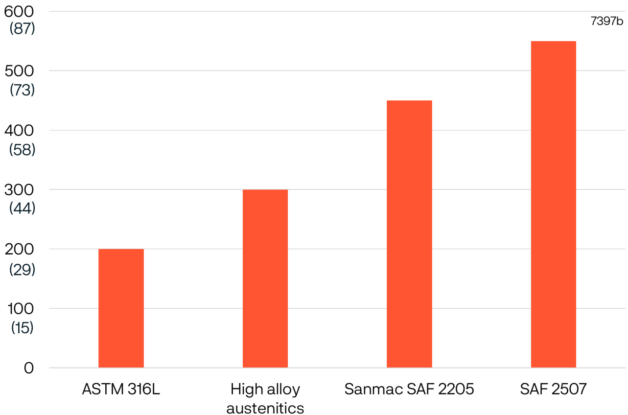
Figure 2. Typical proof strength (Rp0.2) values, comparison
