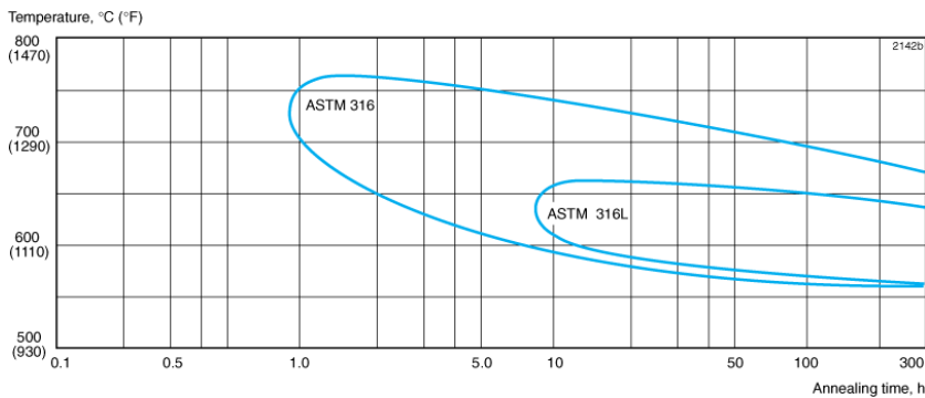
Figure 2. TTC-diagram for Sandvik 3R60 (AISI 316L) and AISI 316. Pitting and crevice corrosion
